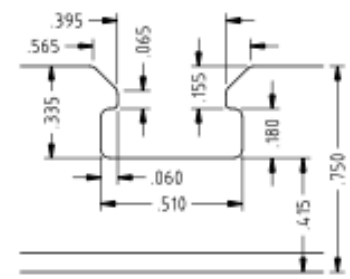
DETAIL "B" *PUNCHED THROUGH BOTH SIDES*
