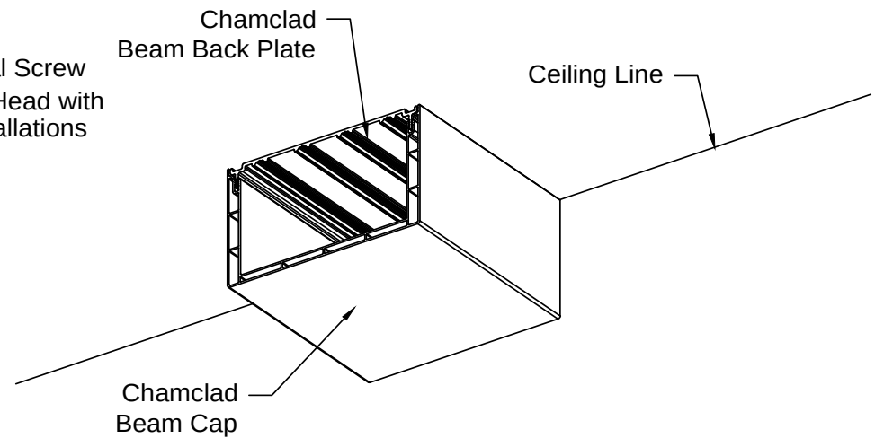
2 CD-18 CHAMCLAD BEAM SYSTEM ISOMETRIC VIEW NOT TO SCALE:
