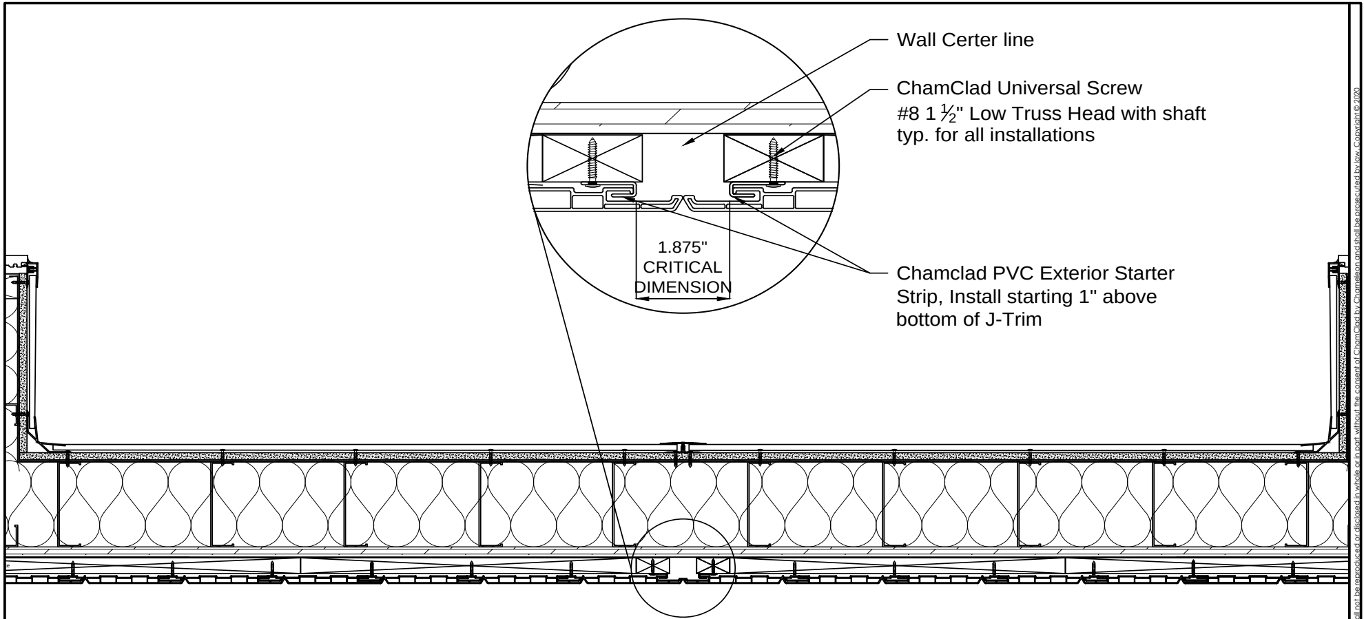
1 CD-10 CHAMCLAD WALL SYSTEM WALL CENTER DETAIL NOT TO SCALE:
