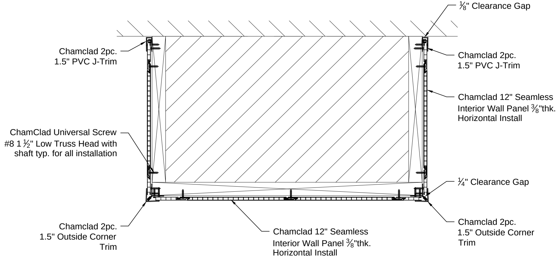
CHAMCLAD BEAM SYSTEM 1 CD-16 NOT TO SCALE
