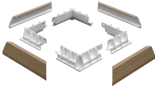
QUICK CLICK COLUMN CAP OR BASE TRIM FOR 7" AND 8" COLUMNS
